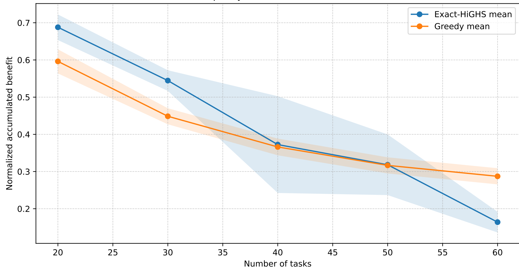
Solution quality across scaled TTAP instances
